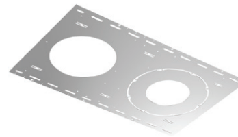
Multi-fit Plate 6" to 10" Holes for Stud Ceiling
